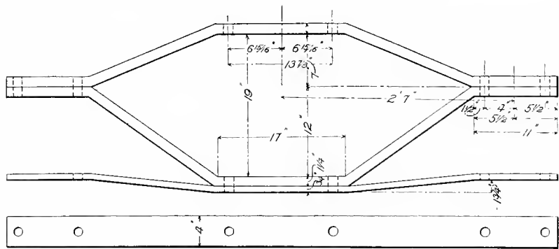
Figs. 4587-4590. UPPER AND LOWER ARCH-BARS AND TIE-BAR.
